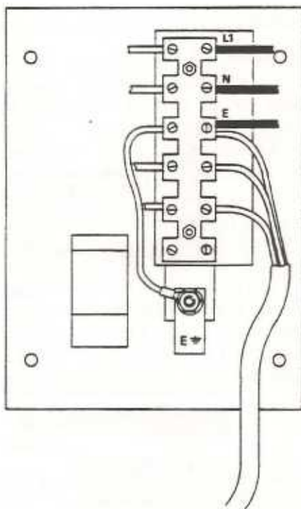
SINGLE PHASE
