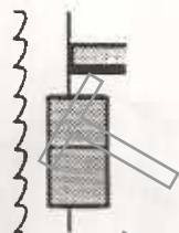
INCORRECT Insufficient support for blade from guide.
