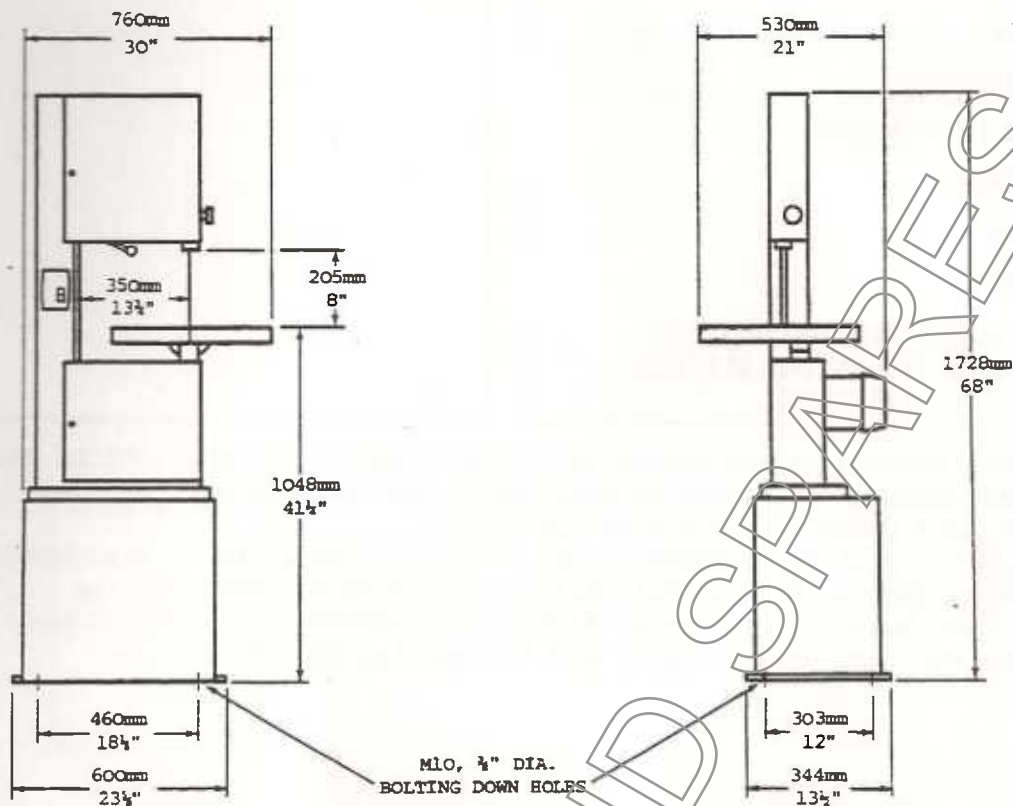
FOUNDATION PLAN FOR MODEL 351 BANDSAWING MACHINE.
